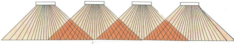
Figure 3 Overlapping patterns with many LED light fixtures
