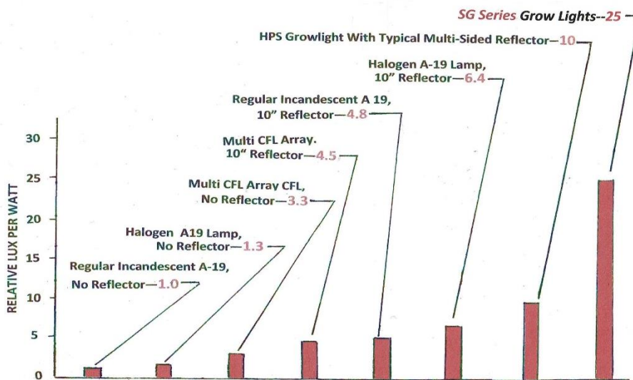
Figure 8 Comparison of High Wattage Lighting Methods
